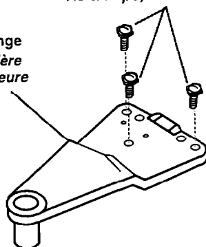
5/16" hex screws Vis 5/16 po, tête hexagonale
